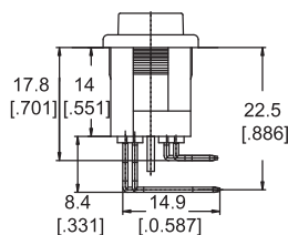
Right Angle PC Through Hole Terminal
