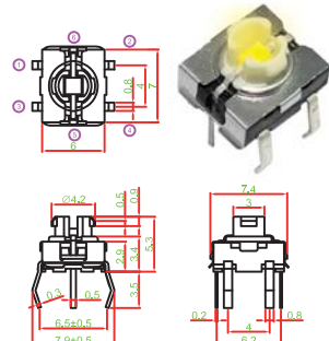
TC009L-N11AA1AX□□□□
