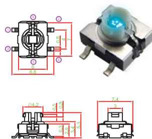
TC009L-N11AAAX□□□□
