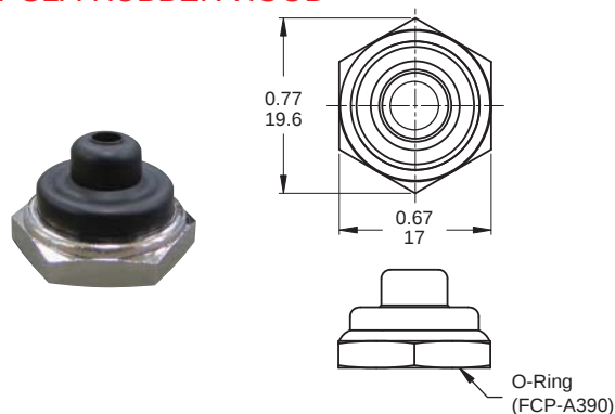
PG2A-RUBBER-HOOD
