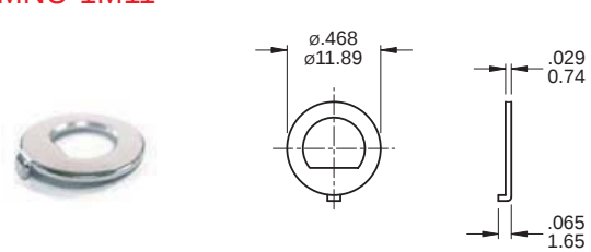
MNU-1M11
