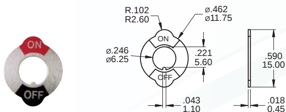
MNU-1M10
